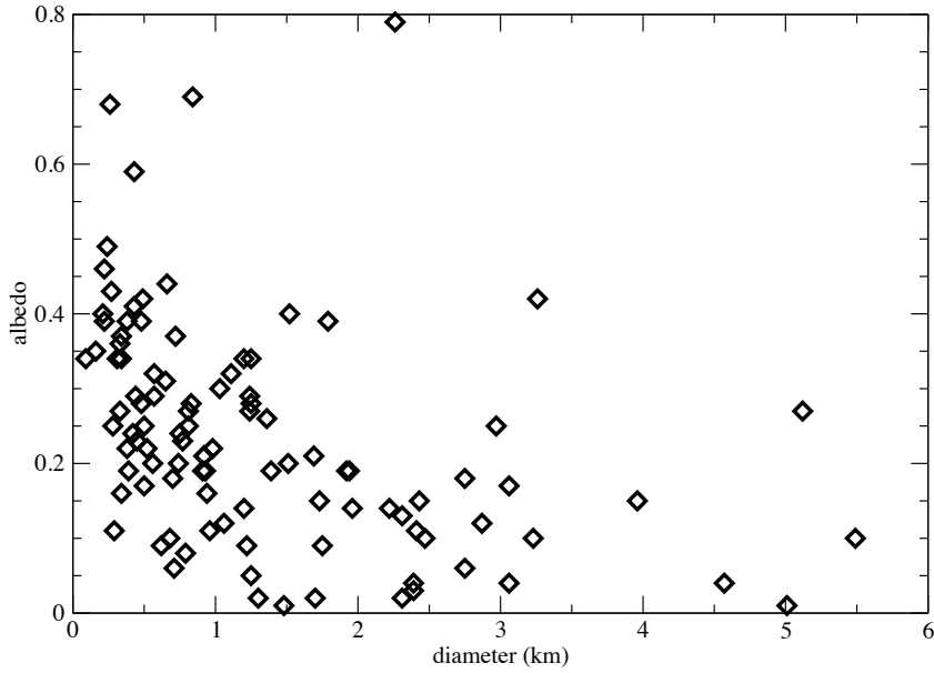
Fig. 4.— Albedo versus diameter for our first 100 targets, using fixed \eta solutions in all cases. Two objects are off the plot: 42286 (2001 TN41), with modeled p_V of 1.03 and diameter 0.7 km, and (433) Eros, with modeled p_V of 0.06 and diameter 32 km; see §5.3 for discussion of these objects.
