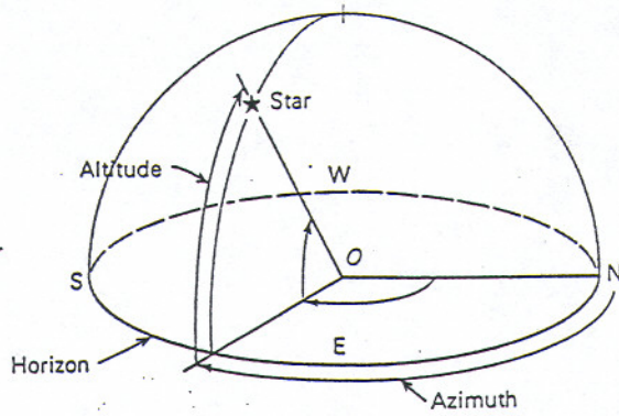
FIG. 7-5 Altitude and azimuth.
