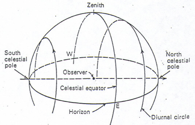
FIG. 7-8 Sky from the equator.
