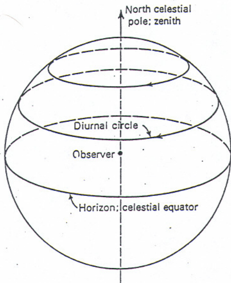
FIG. 7-7 Sky from the North Pole.
