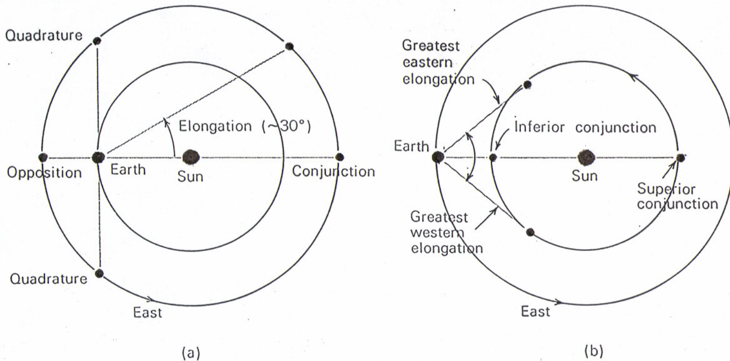
FIG. 3-3 (a) Configurations of a superior planet; (b) configurations of an inferior planet.
